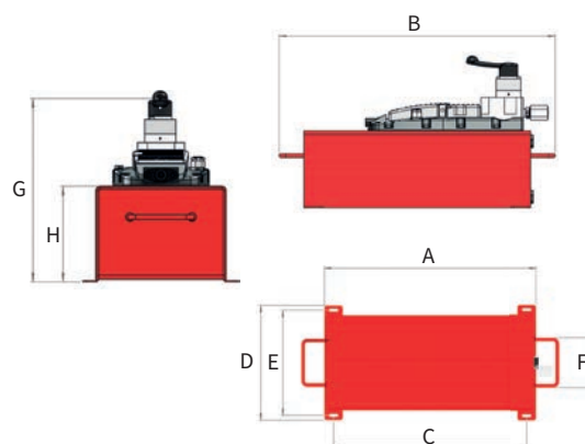
AHP1122, AHP1142(钢制油箱)
