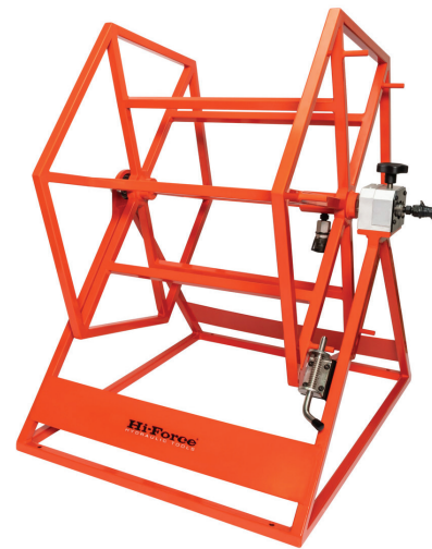
Dimensions Length 800 mm x Width 600 mm x Height 870 mm
