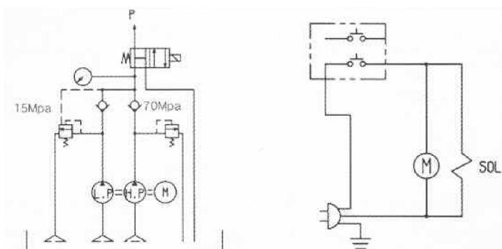
HEP103241S AN HEP103242S CIRCUITS
