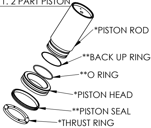
FIG 1. 2 PART PISTON
