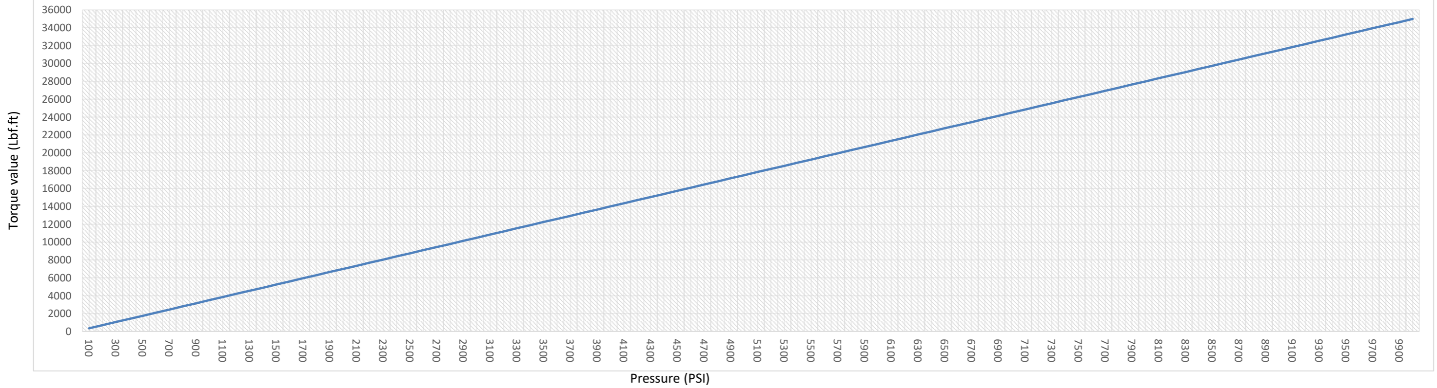
TWH430N Torque/Pressure Conversion Chart (Lbf.ft/PSI) Hex link AF Range 5" to 6.7/8" (130mm to 175mm)
