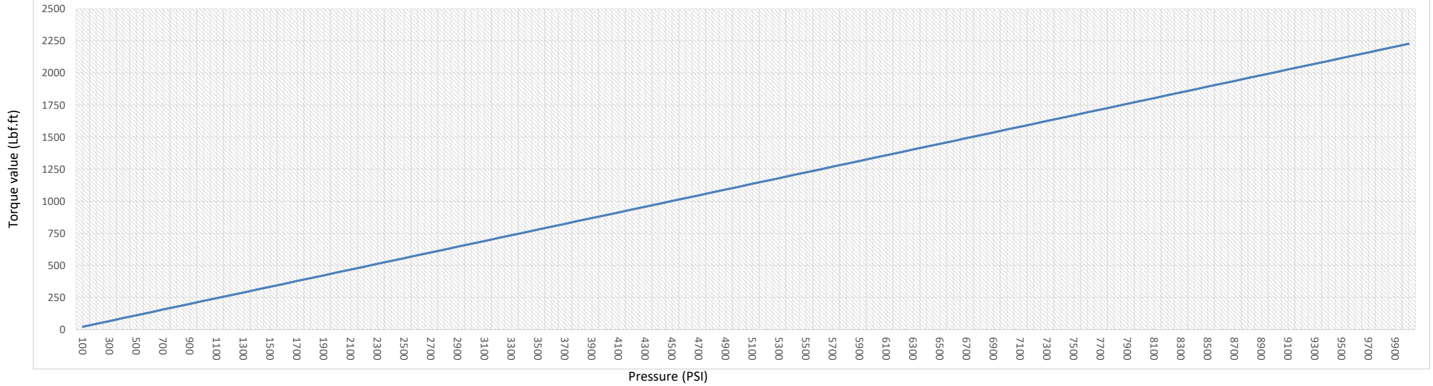
TWH27N Torque/Pressure Conversion Chart (Lbf.ft/PSI) Hex link AF Range 2" to 2.3/8" (50mm to 60mm)
