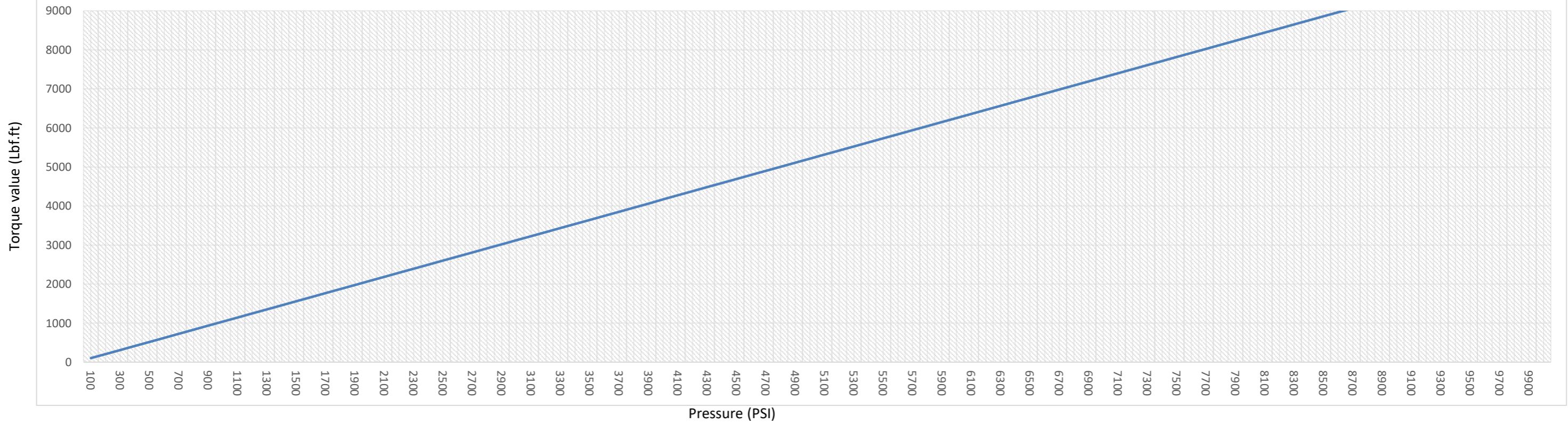
TWH120N Torque/Pressure Conversion Chart (Lbf.ft/PSI) Hex link AF Range 3.1/2" to 3.7/8" (85mm to 100mm)
