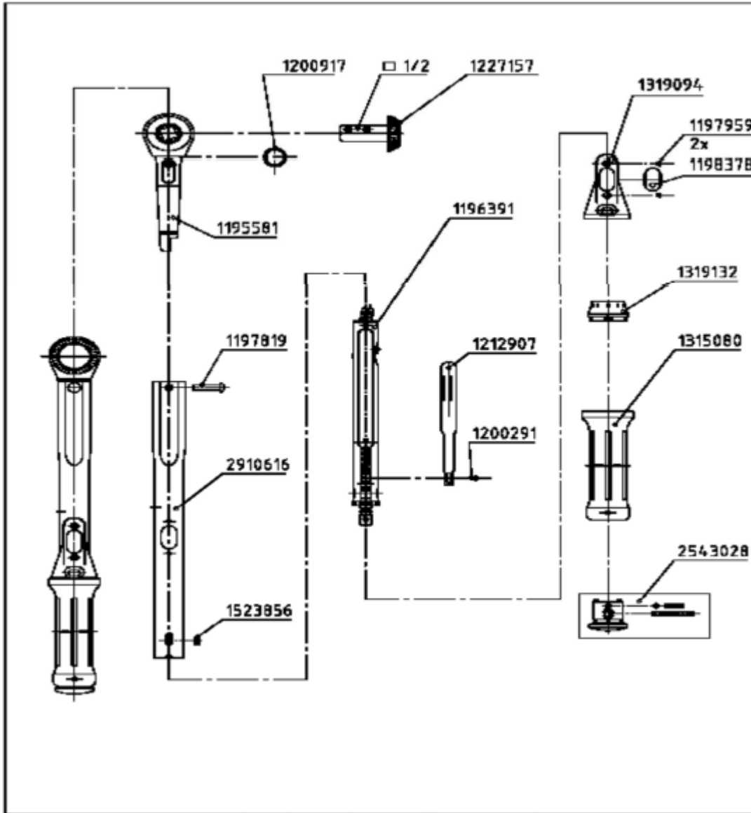
HI-FORCE MANUAL TORQUE WRENCH SPARE PARTS BREAKDOWN SHEET FOR TWM100
