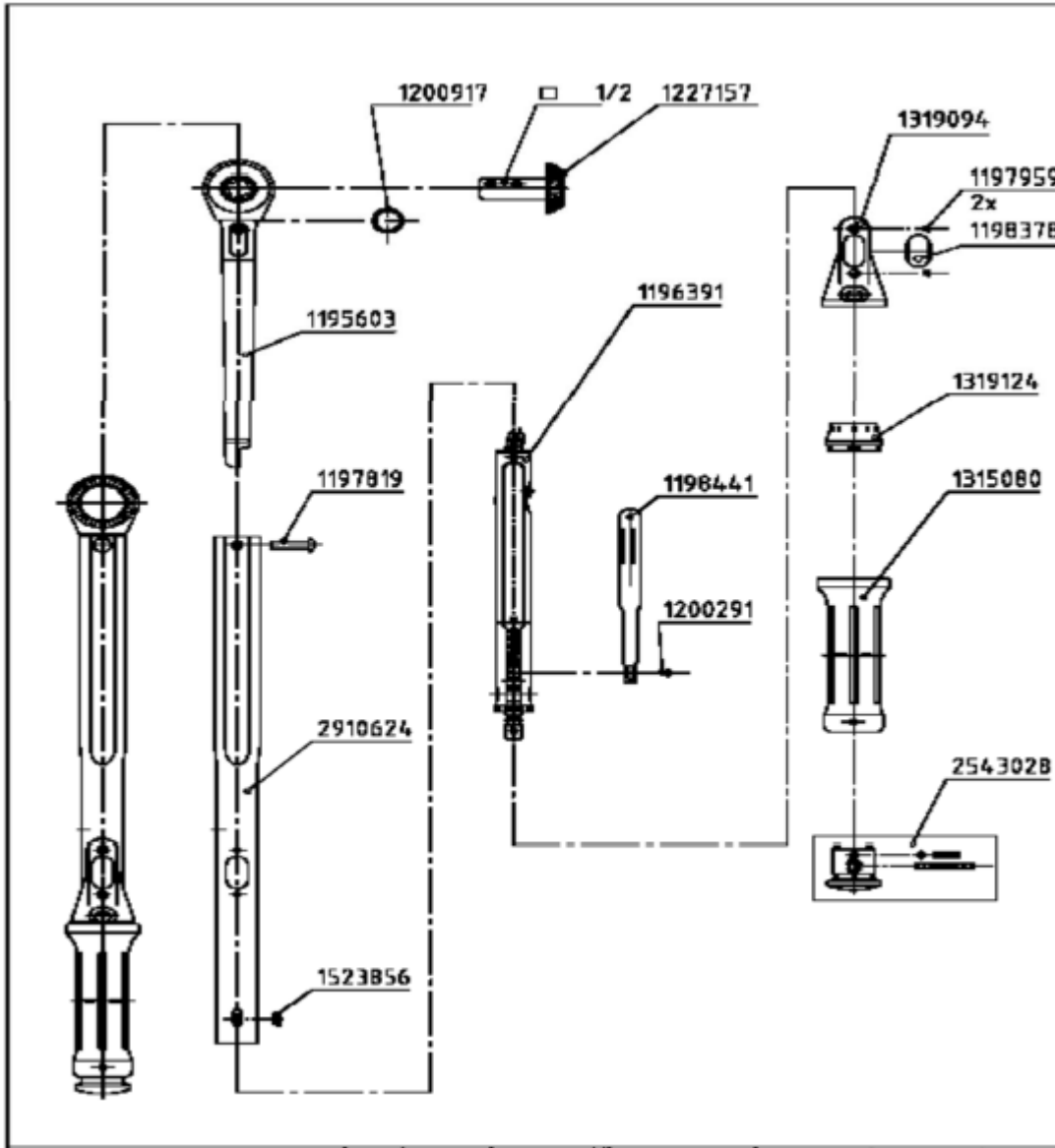
HI-FORCE MANUAL TORQUE WRENCH SPARE PARTS BREAKDOWN SHEET FOR TWM200
