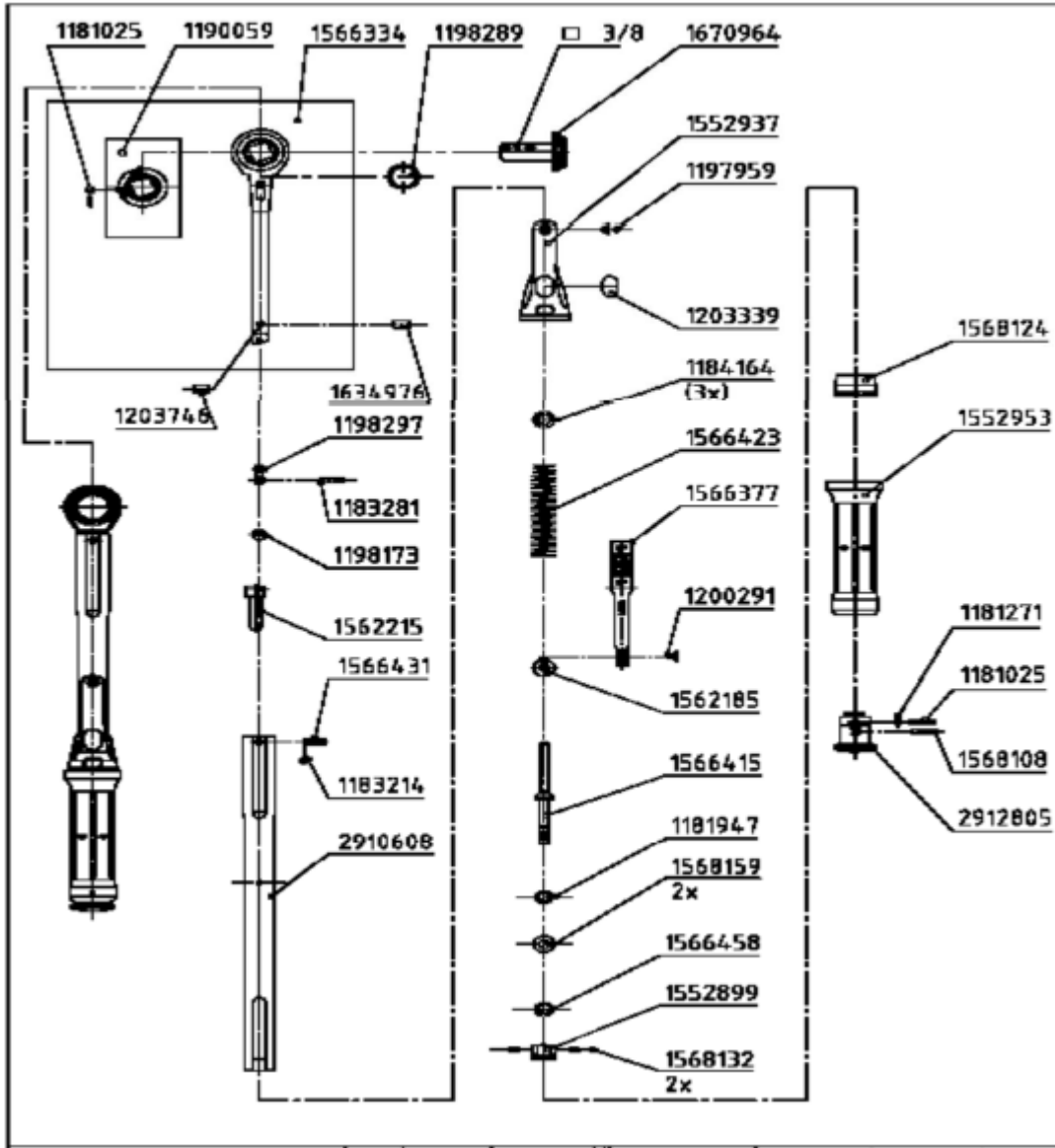
HI-FORCE MANUAL TORQUE WRENCH SPARE PARTS BREAKDOWN SHEET FOR TWM50
