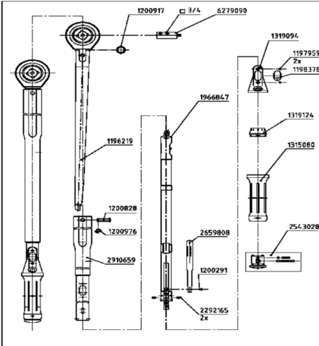
HI-FORCE MANUAL TORQUE WRENCH SPARE PARTS BREAKDOWN SHEET FOR TWM550
