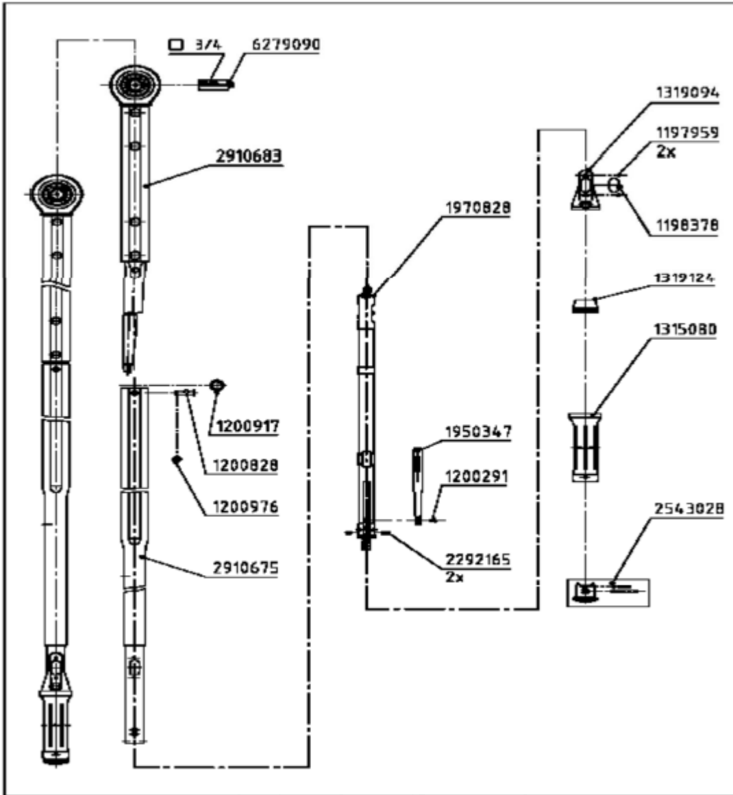
HI-FORCE MANUAL TORQUE WRENCH SPARE PARTS BREAKDOWN SHEET FOR TWM850
